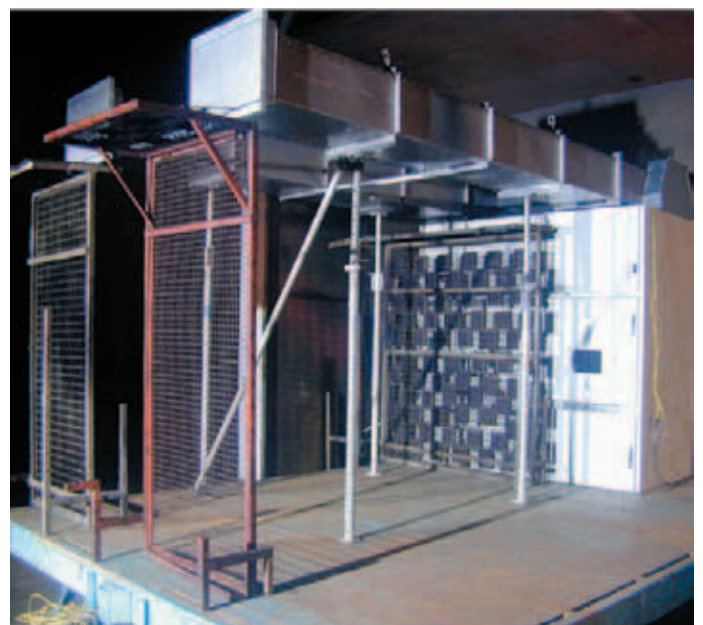
Figure 2: UniGear ZS1 during internal arc test
