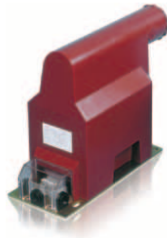
Figure 34: Single-pole VTs with fuse - type TJP
