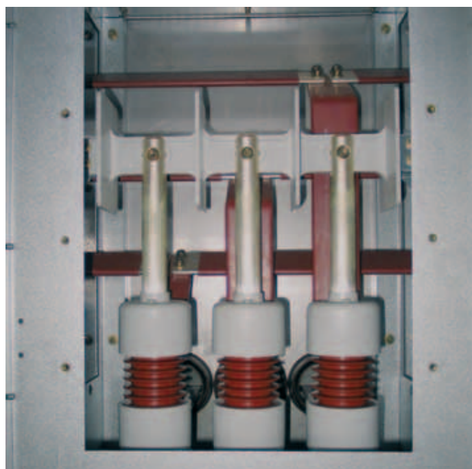
Figure 64: Open position of busbar-disconnector
