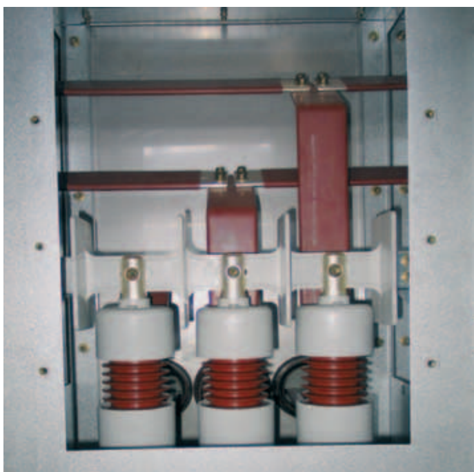
Figure 63: Closed position of busbar-disconnector
